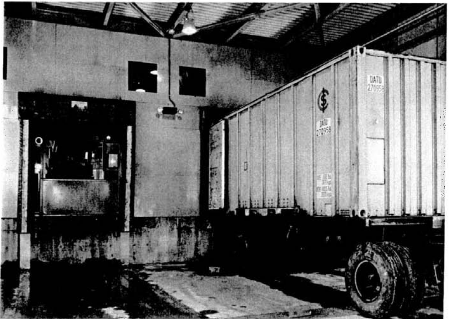
A 20-foot-long by eight-foot-wide by eight-foot-high container in position at one of the two loading docks in the shipping section of the matte processing plant. The end of the retractable conveyor can be seen at the empty dock. Note the metric gross weight of 20,320 kilograms, marked on the container!
