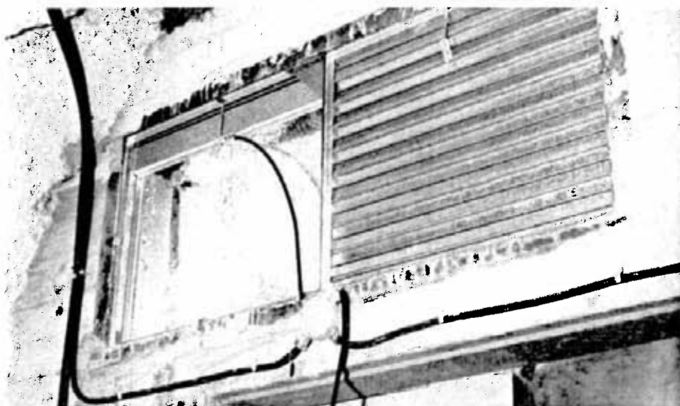
Two fireproof dampers ventilate the vault. The damper at left is in the normal open position, while the damper at right demonstrates the closed position, resulting from the first sensor being activated.
